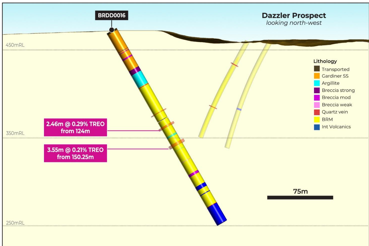
Figure 7: Cross section facing north-west illustrating the Dazzler DD (thick) with previously drilled holes (thinner) by lithology. TREO \geq 0.15% is illustrated as translucent red halos around holes.
